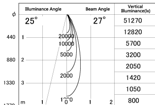
■ Direct Horizontal Illuminance DD126-4025MW9027-LX
