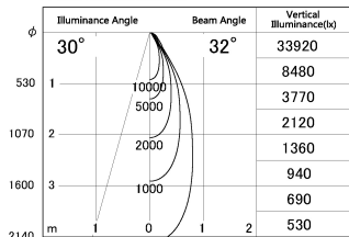
■ Direct Horizontal Illuminance DD126-4035MW9027-LX
