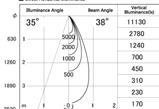
■ Direct Horizontal Illuminance DD126-1435MW9027-LX
