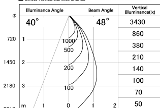
■ Direct Horizontal Illuminance DD126-0855MW9027-LX
