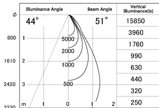
■ Direct Horizontal Illuminance DD126-3755MW9030-LX
