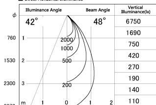
■ Direct Horizontal Illuminance DD126-1455MW9030-LX
