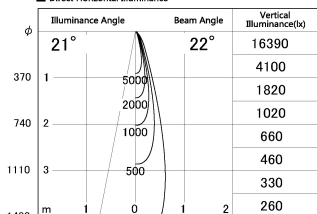
■ Direct Horizontal Illuminance DD126-0825MW9030-LX
