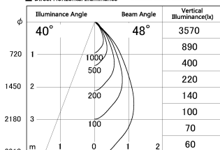
■ Direct Horizontal Illuminance DD126-0855MW9030-LX
