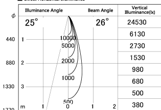
■ Direct Horizontal Illuminance DD126-1425MW9035-LX
