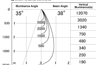
■ Direct Horizontal Illuminance DD126-1435MW9035-LX
