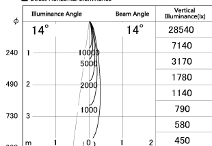
■ Direct Horizontal Illuminance DD126-0815MW9035-LX
