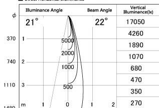
■ Direct Horizontal Illuminance DD126-0825MW9035-LX
