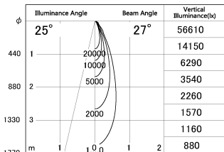
■ Direct Horizontal Illuminance DD126-4025MW9040-LX
