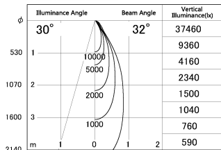
■ Direct Horizontal Illuminance DD126-4035MW9040-LX
