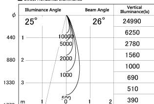
■ Direct Horizontal Illuminance DD126-1425MW9040-LX
