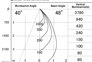
■ Direct Horizontal Illuminance DD126-0855MW9040-LX
