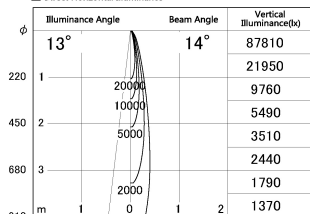
■ Direct Horizontal Illuminance DD126-2515MB9027-LX
