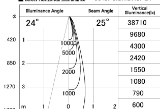
■ Direct Horizontal Illuminance DD126-2525MB9027-LX
