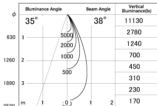
■ Direct Horizontal Illuminance DD126-1435MB9027-LX
