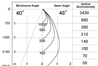
■ Direct Horizontal Illuminance DD126-0855MB9027-LX
