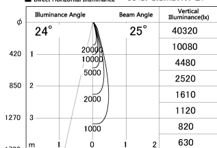
■ Direct Horizontal Illuminance DD126-2525MB9030-LX
