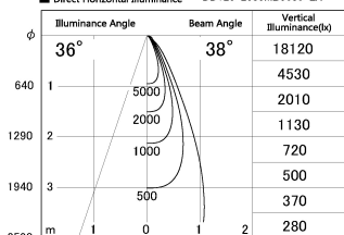
■ Direct Horizontal Illuminance DD126-2535MB9030-LX
