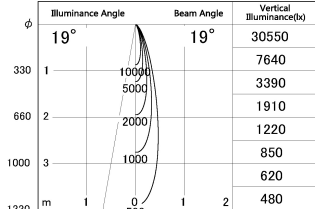
■ Direct Horizontal Illuminance DD126-1415MB9030-LX
