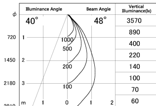
■ Direct Horizontal Illuminance DD126-0855MB9030-LX
