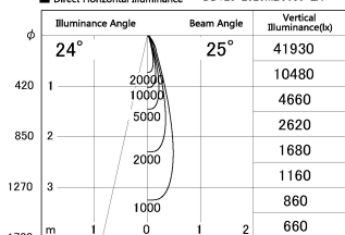
■ Direct Horizontal Illuminance DD126-2525MB9035-LX
