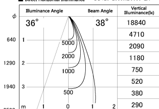
■ Direct Horizontal Illuminance DD126-2535MB9035-LX
