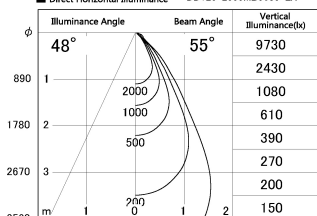
■ Direct Horizontal Illuminance DD126-2555MB9035-LX
