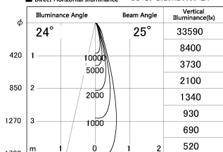
■ Direct Horizontal Illuminance DD126-2025MB9035-LX
