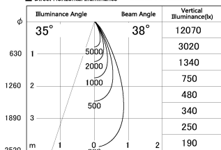
■ Direct Horizontal Illuminance DD126-1435MB9035-LX
