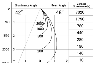
■ Direct Horizontal Illuminance DD126-1455MB9035-LX
