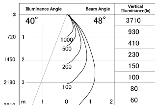
■ Direct Horizontal Illuminance DD126-0855MB9035-LX
