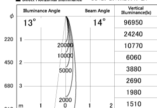
■ Direct Horizontal Illuminance DD126-2515MB9040-LX
