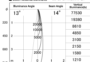
■ Direct Horizontal Illuminance DD126-2015MB9040-LX
