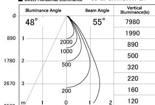
■ Direct Horizontal Illuminance DD126-2055MB9040-LX
