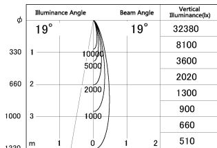
■ Direct Horizontal Illuminance DD126-1415MB9040-LX
