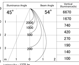
■ Direct Horizontal Illuminance SD359-1450B9035-IN
