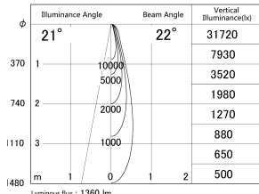
■ Direct Horizontal Illuminance SD359-1420W9030
