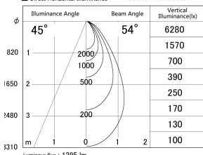
■ Direct Horizontal Illuminance SD359-1450B9027
