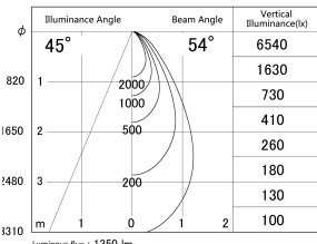
■ Direct Horizontal Illuminance SD359-1450B9030
