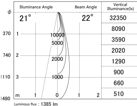
■ Direct Horizontal Illuminance SD359-1420B9035
