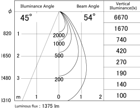
■ Direct Horizontal Illuminance SD359-1450B9035
