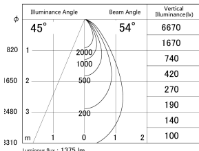
■ Direct Horizontal Illuminance SD359-1450W9035-IK
