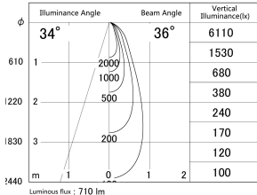
■ Direct Horizontal Illuminance DD133-0835W9027
