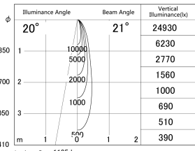
■ Direct Horizontal Illuminance DD161-1020B9027
