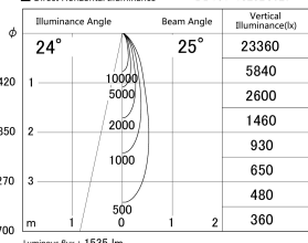
■ Direct Horizontal Illuminance DD161-1525B9027
