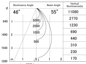
■ Direct Horizontal Illuminance DD161-2555B9027
