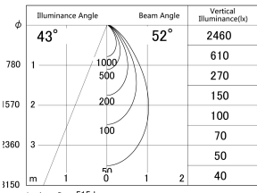
■ Direct Horizontal Illuminance DD161-0550B9030
