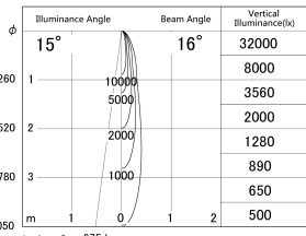
■ Direct Horizontal Illuminance DD161-1015B9030
