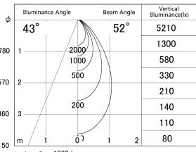
■ Direct Horizontal Illuminance DD161-1050B9030
