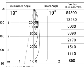
Direct Horizontal Illuminance DD161-2520B9030
